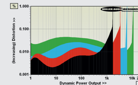
ABOVE: Dynamic power output versus distortion into 80hm (black trace), 40hm (red), 20hm (blue) and 1ohm (green) speaker loads. Max. current is 106A (!)
