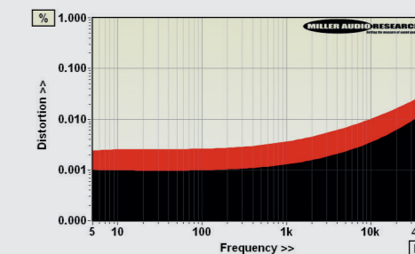
ABOVE: Distortion versus extended frequency (1W/80hm, black; 100W/80hm, red)
